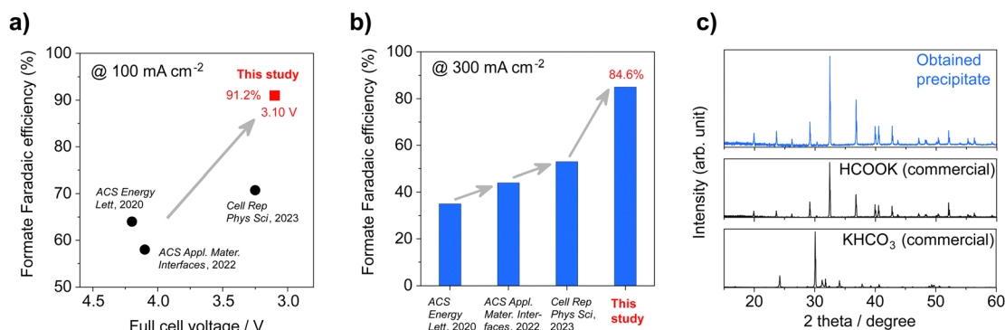
Fig. 6 Comparison of performances with literature on bicarbonate electrolyzers for formate synthesis: (a) formate FE and full cell voltage at 100\text{ mA cm}^{-2} and (b) formate FE at 300\text{ mA cm}^{-2} (except for Cell Rep. Phys. Sci. , 2023 at 200\text{ mA cm}^{-2} ). (c) Powder XRD patterns of the precipitate obtained by evaporating the catholyte after the bicarbonate electrolyzer reaction (Fig. S10, ESI † ) and commercial salts of \text{HCOOK} and \text{KHCO}_3 .
